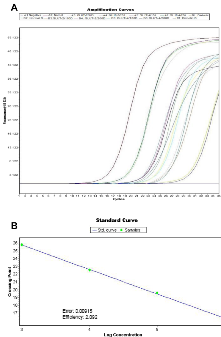
Fig. 3 Simultaneous amplification plots and standard curves of GLUT-2 & 4 mRNA by fluorescence real-time PCR. a. Plot of threshold cycle number (Ct) vs. serial dilutions (log 10 ) of standard DNA from 10 1 to 10 8 copies/reaction tube were prepared. Reaction number increases during PCR as the amplicon copy number increases until the reaction reaches a plateau. Ct was plotted against each copy number. Ct represents the PCR cycle at which reporter signal can first be detected. b. Standard curve showing efficiency of amplification during PCR
