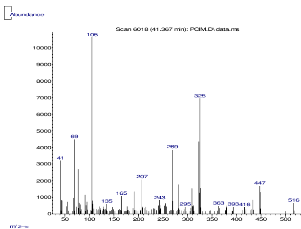
Figure 3 Mass spectra peaks (m/z) of sub-fraction I obtained by GC-MS.
